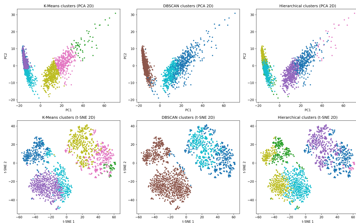
Figure 6: PCA (top row) and t-SNE (bottom row) projections colored by cluster assignment for K-Means, DBSCAN and Hierarchical (Ward) respectively.
